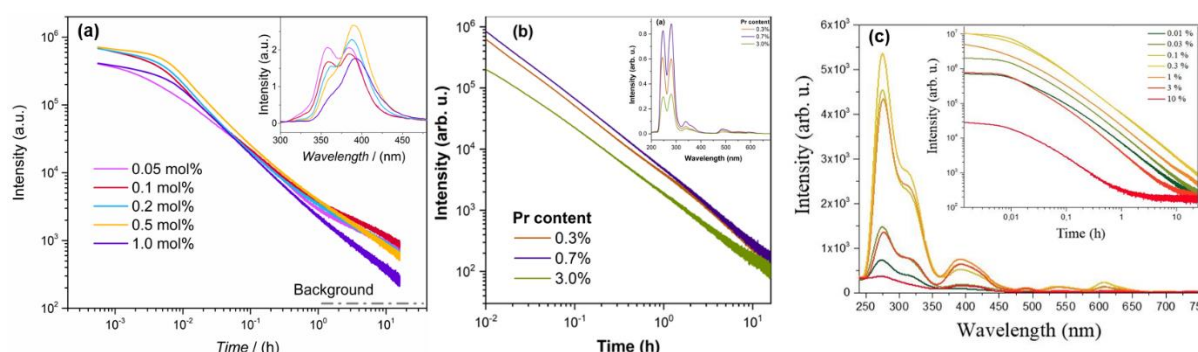
Fig. 1. Decay kinetics and persistent luminescence spectra of a) \text{Sr}_3\text{MgSi}_2\text{O}_8: \text{Ce}^{3+} b) \text{Sr}_2\text{MgSi}_2\text{O}_7: \text{Pr}^{3+} and c) \text{Ca}_2\text{Al}_2\text{SiO}_7: \text{Pr}^{3+} .
