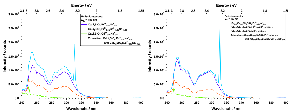
Fig. 1. Up-conversion emission spectra of \text{CaLi}_2\text{SiO}_4 doped with \text{Pr}^{3+} , with \text{Gd}^{3+} , or with both of them. All materials are also doped by \text{Na}^+ for the sake of charge compensation. Spectra were recorded upon excitation of 488 nm Laser (75 mW).
