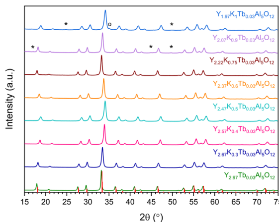
Fig. 1. XRD diffraction patterns of \text{Y}_{2.97-x}\text{K}_x\text{Tb}_{0.03}\text{Al}_5\text{O}_{12} samples. The crystalline phases are marked: vertical red lines - \text{Y}_3\text{Al}_5\text{O}_{12} , * – \text{YAlO}_3 , o – \text{Al}_2\text{O}_3
