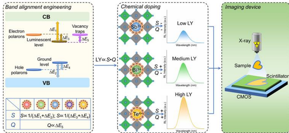
Fig. 1. Schematic diagram for novel design strategy including band alignment engineering, chemical doping and X-ray imaging device, where \Delta E_1 and \Delta E_2 are differences between valence/conduction bands and luminescent centers, \Delta E_3 and \Delta E_4 are differences between STE states and luminescent centers, \Delta E_5 is difference between vacancy traps and luminescent centers.
