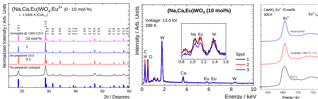
Fig (from left to right): Experimental and calculated XRPD patterns, EDX spectra, and Eu ( \text{L}_{\text{III}} ) XANES spectra for the (\text{Na,Ca,Eu})\text{WO}_4 powders coprecipitated @ 300 K.
