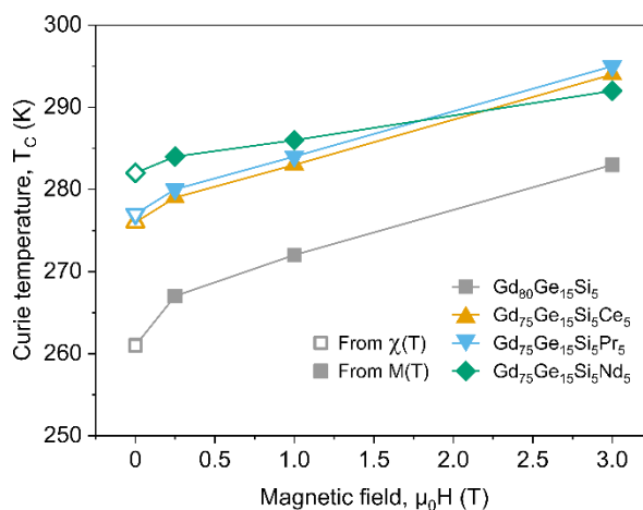
Fig. 1. Curie temperature as a function of applied magnetic field for \text{Gd}_{75}\text{Ge}_{15}\text{Si}_5\text{X}_5 alloys, where \text{X} = \text{Ce}, \text{Pr}, \text{or Nd} , determined from the M(T) and \chi(T) measurements.
