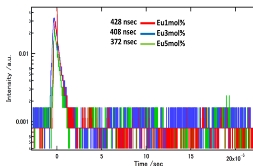
Fig.3 Scintillation decay curves under 662keV gamma-ray irradiation.
