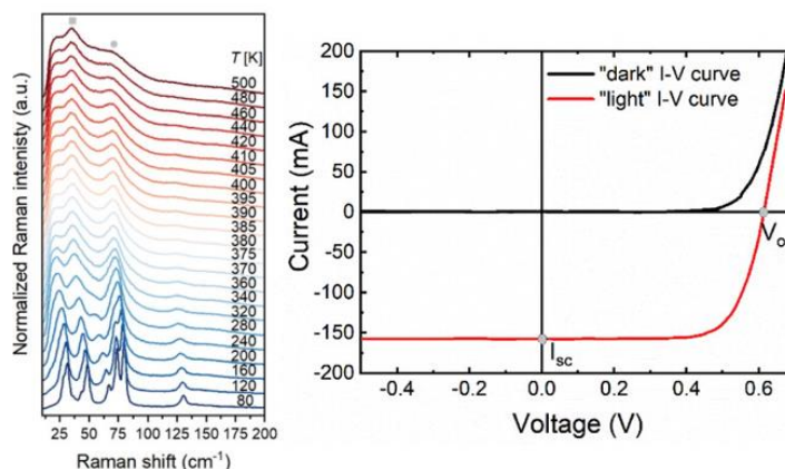
Fig. 1. Thermal evolution of Raman spectra obtained for \text{CsPbBr}_3:\text{Yb}^{3+} (left) and I - V characteristics for the solar cell with \text{CsPbBr}_3:\text{Yb}^{3+} thin layer in dark and under illumination. Figures are licensed under CC BY 4.0 [5].
