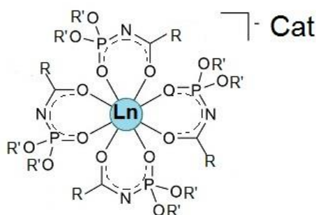
Fig. 1. General structural formula of Cat[LnL 4 ] complexes.
